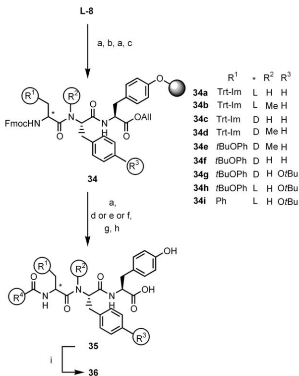
Scheme 4. (a) Piperidine/DMF 1/4, 2×5 min or 2×20 min; (b) 27 , HATU, i PrNEt 2 , NMP, 2.5 h; (c) 27 , HATU, i PrNEt 2 , NMP or DIC, HOAt, DMF, 14 h; (d) 29 , HATU, HOAt, i PrNEt 2 , NMP, 12–24 h; (e) 30 , PyAOP, DMAP, i PrNEt 2 , CH 2 Cl 2 /DMF 1/2, 12–24 h; (f) 31 , HOAt, DMAP, i PrNEt 2 , CH 2 Cl 2 /DMF 2/1, 7–10 h; (g) Pd(PPh 3 ) 4 , morpholine, THF, 4–16 h; (h) TFA/H 2 O 95/5, 4–5 h; (i) 10% Pd/C, H 2 , dioxane, 8 h.
