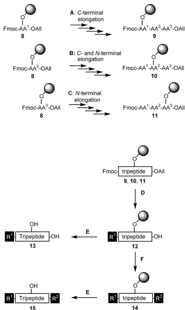
Scheme 2. Planned synthesis of a peptidocinnamin E library.
