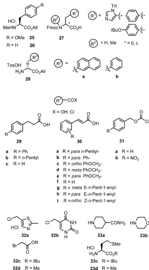
Figure 2. Building blocks used for the solid phase synthesis.
