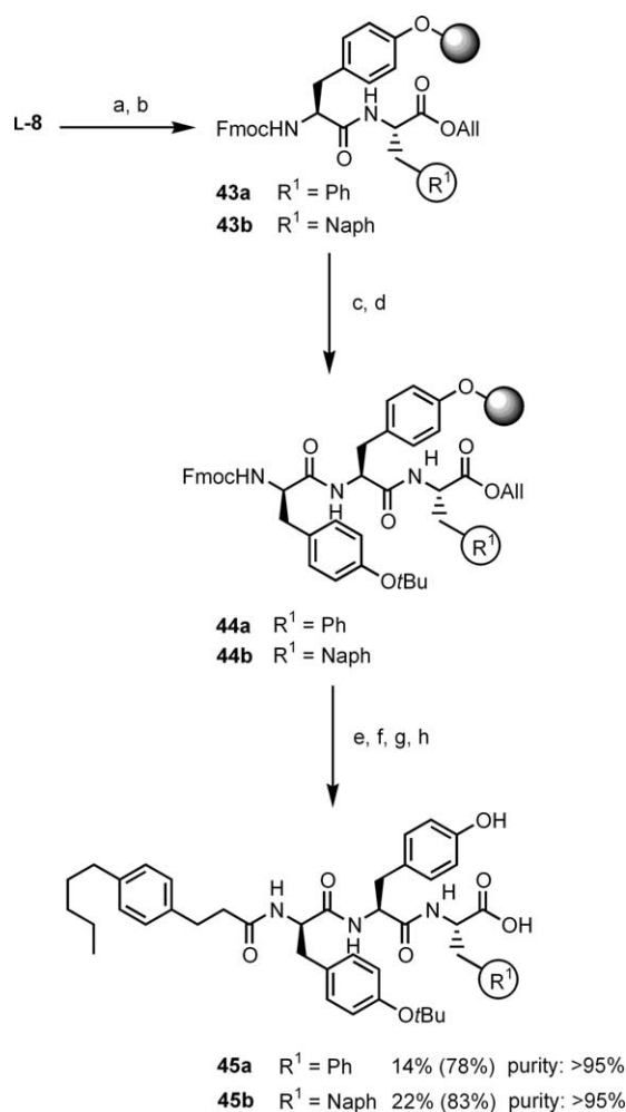
Scheme 6. (a) Pd(PPh 3 ) 4 , NMA, THF; (b) 26 , PyAOP, i PrNEt 2 , NMP, 8 h; (c) piperidine/DMF 1/4, 2×5 min; (d) Fmoc-D-Tyr( t Bu)OH, HATU, i PrNEt 2 , NMP, 14 h; (e) 29 , HATU, HOAt, i PrNEt 2 , NMP, 12 h; (f) Pd(PPh 3 ) 4 , morpholine, THF, 24 h. TFA/H 2 O 95/5, 3.5 h.
