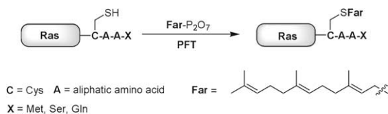
Scheme 1. Farnesylation of Ras-proteins by protein farnesyltransferase (PFT).
