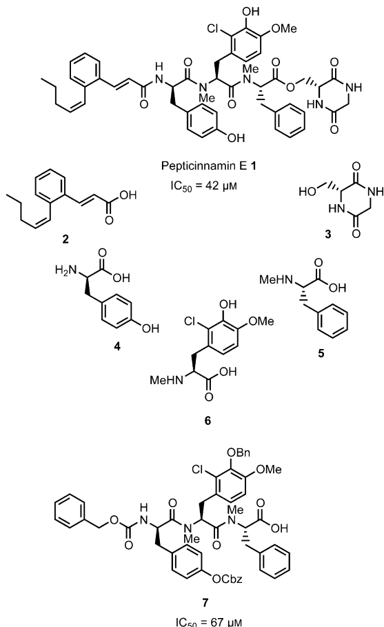
Figure 1. Structure of the farnesyltransferase-inhibitor pepticcinnamin E and its components.
