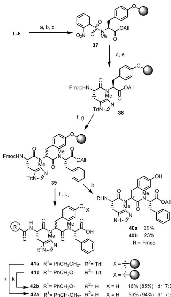
Scheme 5. (a) Piperidine/DMF 1/4, 215 min; (b) o -NO 2 C 6 H 4 SO 2 Cl, lutidine, CH 2 Cl 2 , 11 h; (c) p -NO 2 PhSO 3 Me, MTBD, DMF, 1.5 h; (d) DBU, 2-mercaptoethanol, DMF, 1 h; (e) Fmoc-L-His(Trt)OH, DIC, HOAt, lutidine, DMF, 24 h; (f) Pd(PPh 3 ) 4 , NMA, THF; 24 h; (g) 26 , PyAOP, i PrNEt 2 , NMP, 24 h; (h) 31 , DMAP, HOAt, i PrNEt 2 , DMF/CH 2 Cl 2 , 8 h; (i) 29c , HATU, HOAt, i PrNEt 2 , NMP, 8 h; (j) Pd(PPh 3 ) 4 , morpholine, THF, 24 h; (k) TFA/H 2 O 95/5, 24 h.
