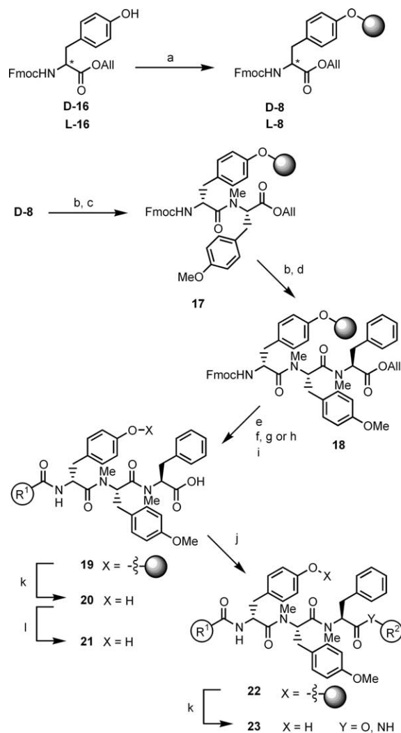
Scheme 3. (a) DEAD, PPh 3 , THF, 0 °C, 1 h, rt, 12 h, loading-level: 0.40–0.53 mmol g -1 , 53–59%; (b) Pd(PPh 3 ) 4 , PhSiH 3 or NMA, THF, 24 h; (c) 25 , HATU, HOAt, i PrNEt 2 , NMP, 48 h; (d) 26 , PyAOP, HOAt, i PrNEt 2 , NMP, 48 h; (e) piperidine/DMF 1/4, 10–40 min; (f) 29 , HATU, HOAt, i PrNEt 2 , NMP, 12–24 h; (g) 30 , PyAOP, DMAP, i PrNEt 2 , CH 2 Cl 2 /DMF 1/2, 12–17 h; (h) 31 , HOAt, DMAP, i PrNEt 2 , CH 2 Cl 2 /DMF 2/1, 7–20 h; (i) Pd(PPh 3 ) 4 , morpholine, THF, 4 h; (j) 33 , PyAOP, i PrNEt 2 , NMP, 16 h (Y = NH); (h) Cs 2 CO 3 , KI, 32 , DMF, 24 h, rt (X = Br) or 24–48 h, 50 °C (X = Cl) (Y = O); (l) TFA/H 2 O 95/5, 4–24 h; (m) 10% Pd/C, H 2 , MeOH, 8 h.
